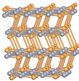
Figure 4. A view of the non-interpenetrated net, jju3 in 4 viewed along the a -axis. The topological representation of the 3D framework created from 2D sheets formed from the tetrahedral Zn1 node (golden yellow) and S -poly-bppcb node (gray) through obc spacer ligand (golden yellow rod).
